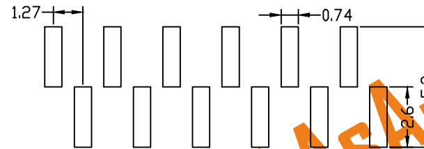
TYPE A PCB LAYOUT
